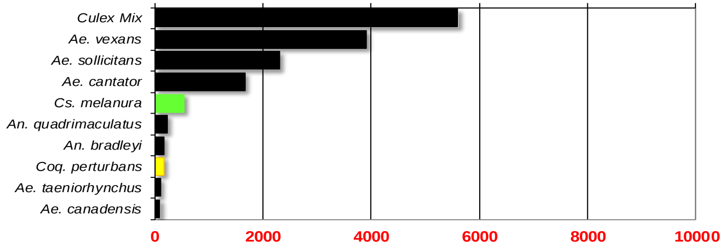
Total # mosquitoes
